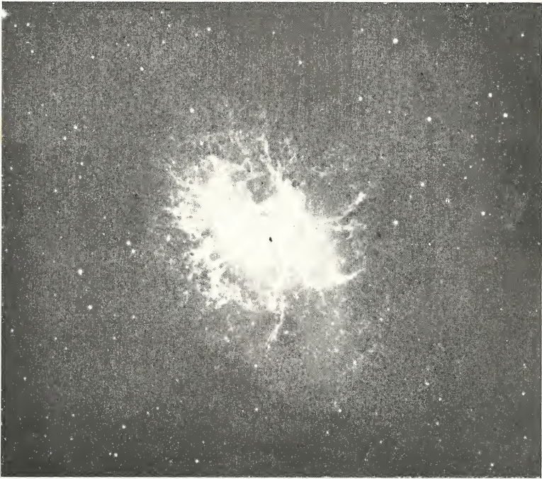
The Crab Nebula in Taurus (By Courtesy of Mt. Wilson and Mt. Palomar Observatories)
